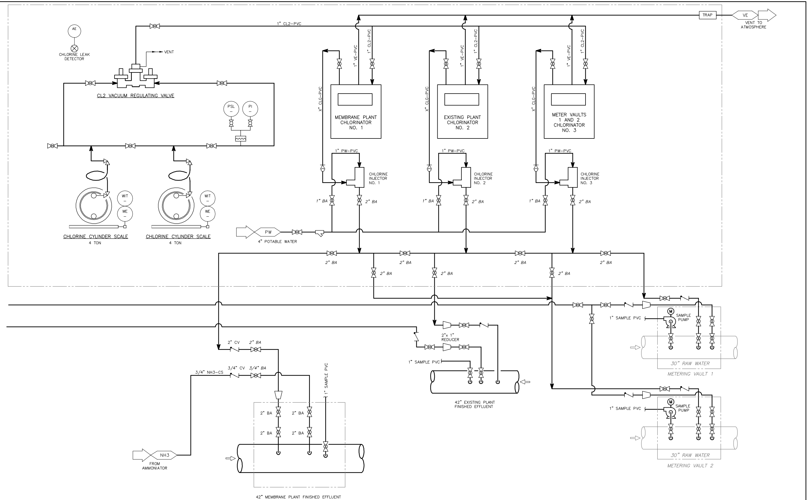
FIGURE 5-30 PM & ID CHLORINE FEED SYSTEM BOSSIER CITY WTP EXPANSION
