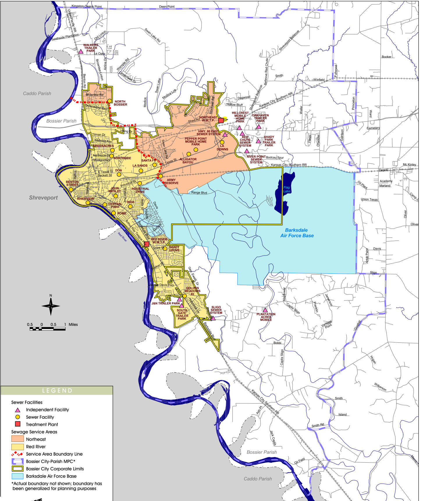
Figure 8.5 Existing Sewer System
