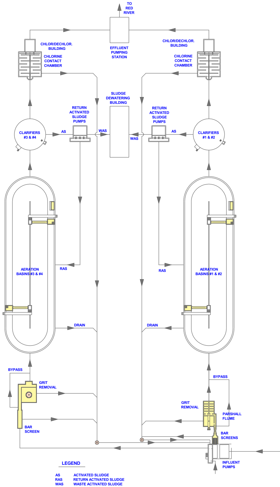
Figure 8.4 Northeast Wastewater Treatment Plant
