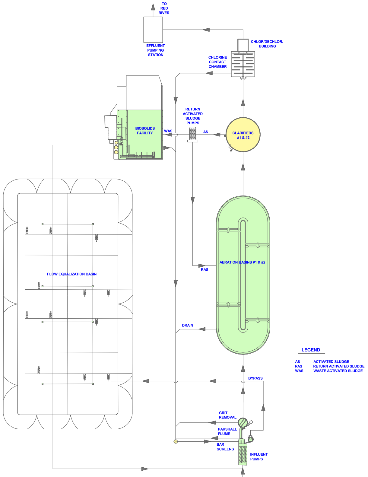
Figure 8.3 Red River Wastewater Treatment Plant Schematic
