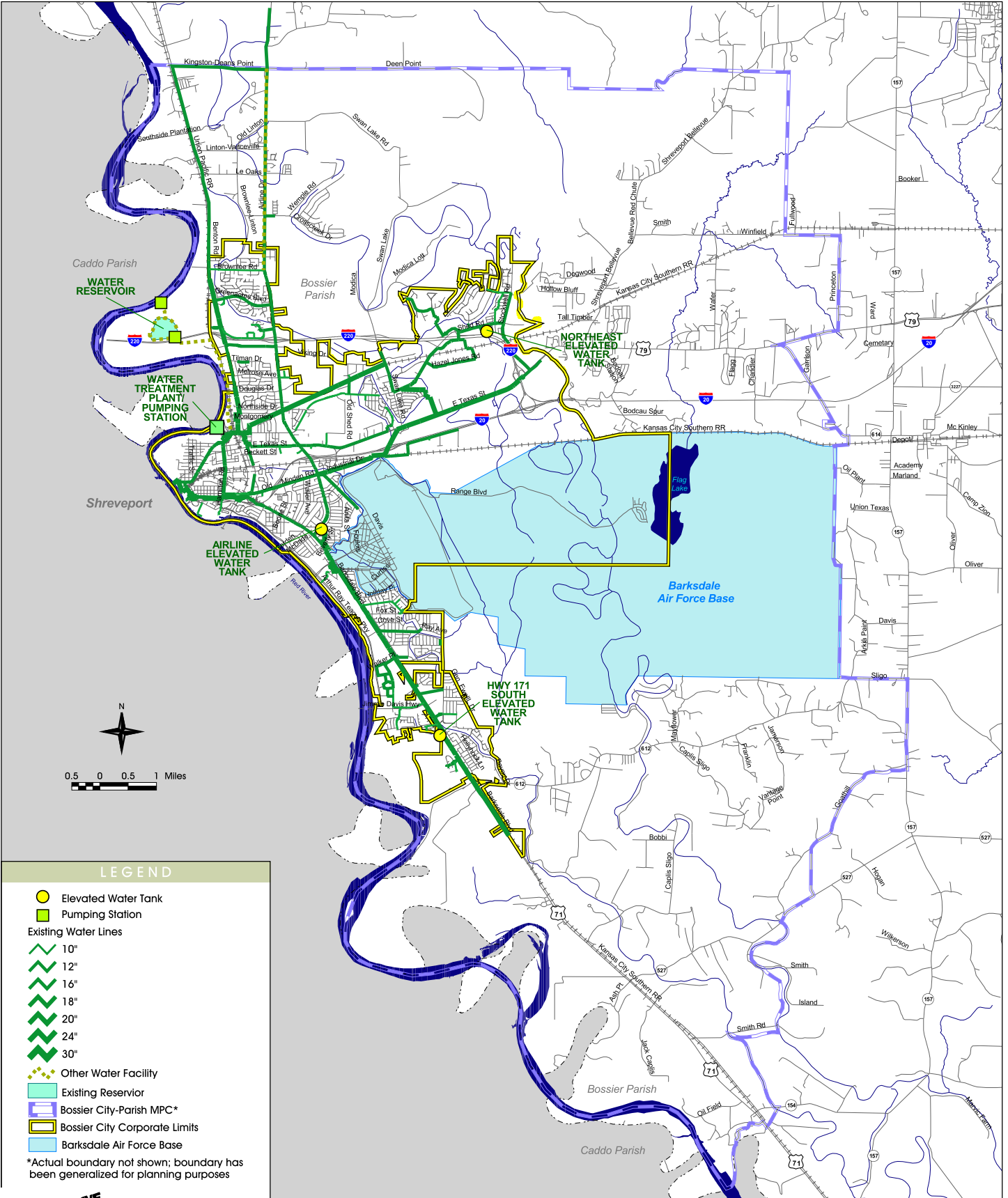
Figure 8.2 Existing Water System
